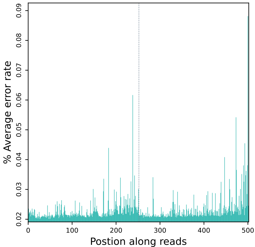
Error rate distribution along reads (R10115)
